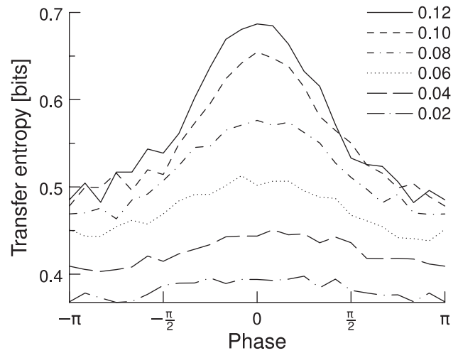
Figure 11. TE as a function of phase shifts and gamma oscillations. If the oscillations are strong in the gamma band ( g_{AMPA}/g_{NMDA} modification ratio=0.12), there is a clear phase shift between the two groups of neurons and the phase dependence curve is clearly bell shaped. If the oscillations are too low, there is no meaningful phase shift and the curve becomes flat ( g_{AMPA}/g_{NMDA} modification ratio=0.02). Averaged over 100 trials. doi:10.1371/journal.pcbi.1000934.g011
