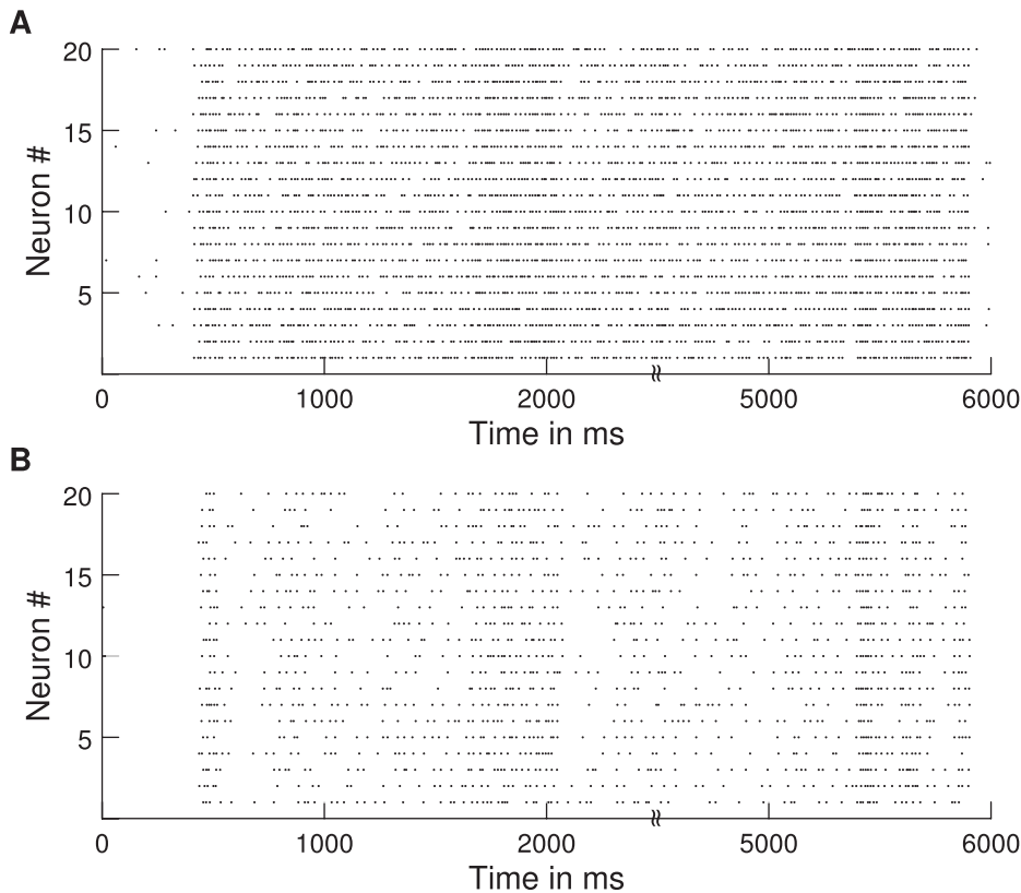
Figure 3. Raster plots. Raster plot of spikes of 20 neurons from the default simulations ( g_{\text{AMPA}}/g_{\text{NMDA}} modification ratio = 0.12). (a) Neurons from selective pool 1. (b) Neurons from selective pool 2. doi:10.1371/journal.pcbi.1000934.g003
