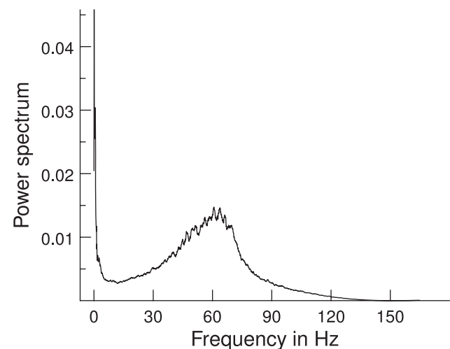
Figure 4. Power spectrum. The power spectrum of the MUA signal from a simulation with default parameters is shown. g_{\text{AMPA}}/g_{\text{NMDA}} modification ratio = 0.12, averaged over 100 trials. doi:10.1371/journal.pcbi.1000934.g004
