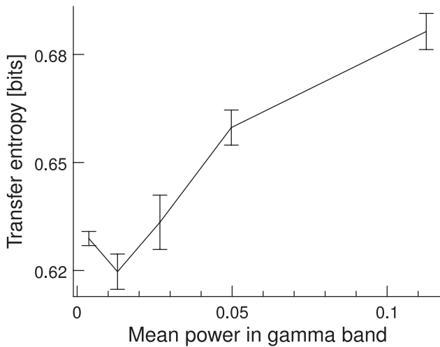
Figure 10. TE of trials sorted by power in the gamma band. Network parameters are kept fixed. The TE increases as a function of gamma power. g_{AMPA}/g_{NMDA} modification ratio=0.12, averaged over 100 trials. Error bars indicate 95% confidence intervals. doi:10.1371/journal.pcbi.1000934.g010
