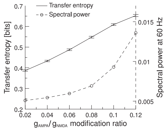
Figure 12. Mean TE as a function of gamma frequency band power. We plot the TE for six different g_{AMPA}/g_{NMDA} modification ratios (solid line). A higher g_{AMPA}/g_{NMDA} modification ratio causes the network to oscillate in the gamma frequency range and thus increases the power in the gamma frequency band (dashed line). Error bars indicate 95% confidence intervals; averaged over 100 trials. doi:10.1371/journal.pcbi.1000934.g012
