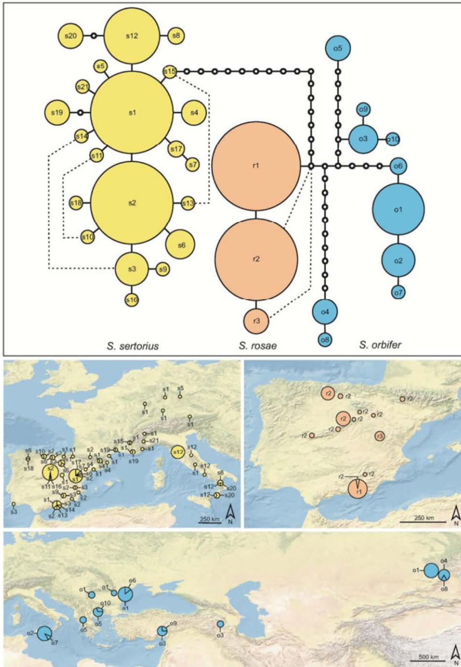
Fig. 1. Mitochondrial COI haplotype networks and their geographical distribution for S. sertorius (yellow), S. rosae sp. nov. (pink) and S. orbifer (blue). The size of the circles is proportional to the number of samples displaying the haplotype. Connections creating loops that are less likely according to frequency and geographic criteria are indicated in dashed lines. Haplotype codes match those in Table S1.
