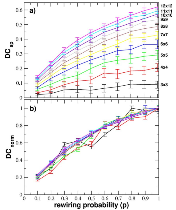
FIG. 2. (Color online) Decision cost DC_{\text{sp}} (a) and normalized decision cost DC_{\text{norm}} (b) of N \times N spatial networks as a function of the rewiring probability p . The number of nodes ranges from 9 ( 3 \times 3 ) to 144 ( 12 \times 12 ). Each point corresponds to the mean value of 20 simulations, with its corresponding error bars.
