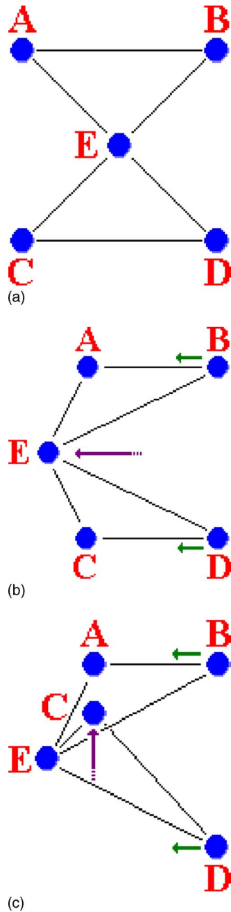
FIG. 1. (Color online) An example of path-searching complexity: a simple net (a) and two evolutions [(b) and (c)]. Depending on the spatial distribution of nodes, the ease of finding the shortest path may change considerably.
