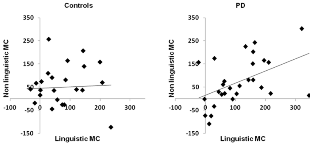
Figure 4. Correlations of the mixing costs of PD patients and controls in the two tasks.
