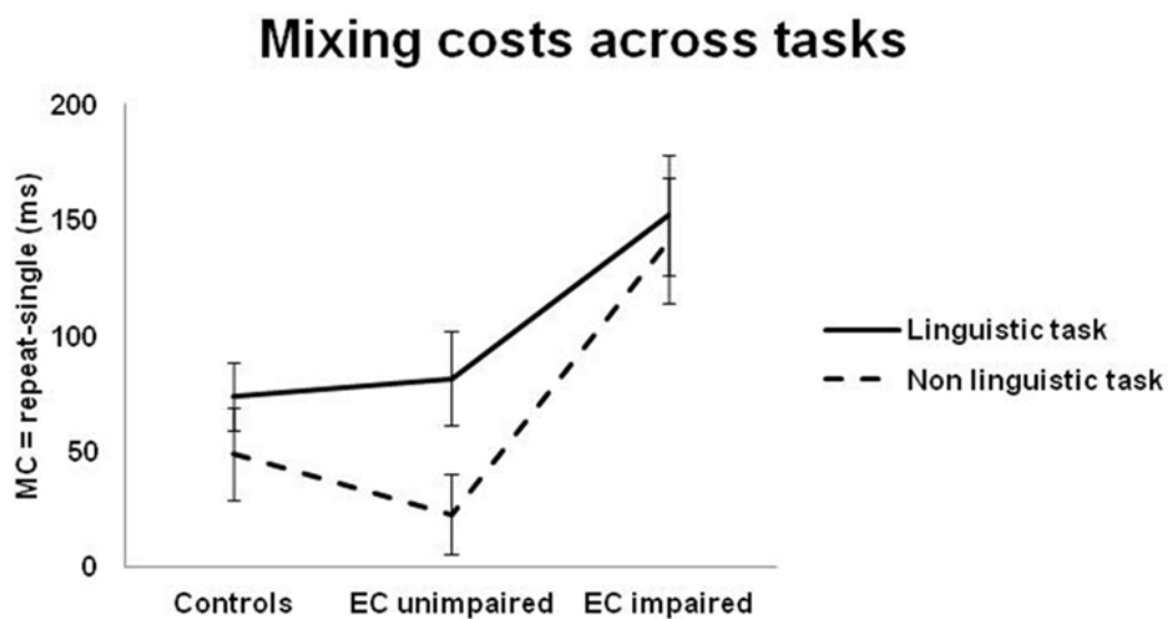
Figure 2. Comparison of the switch and mixing costs of the three groups in the linguistic and non-linguistic task switching.
