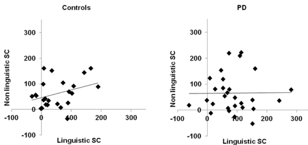
Figure 3. Correlations of the switch costs of PD patients and controls in the two tasks.
