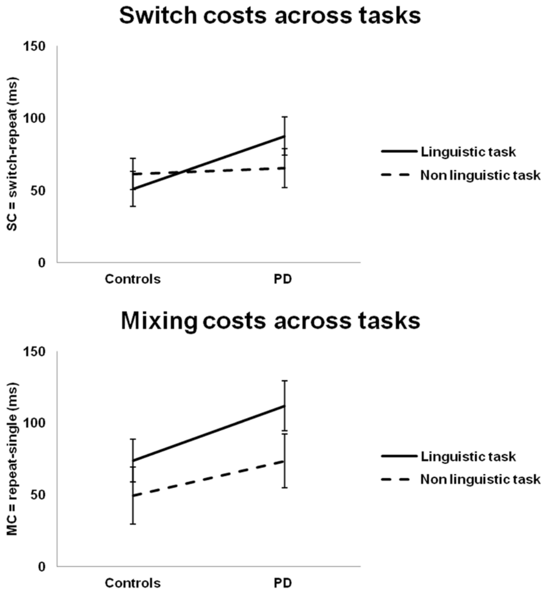
Figure 1. Comparison of the switch and mixing costs of the two groups in the linguistic and non-linguistic task switching.
