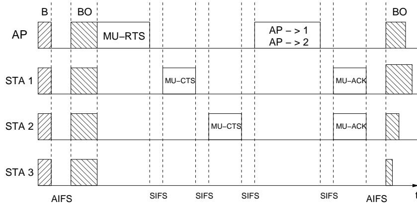
Fig. 4 A successful Uni-MUMAC downlink transmission
