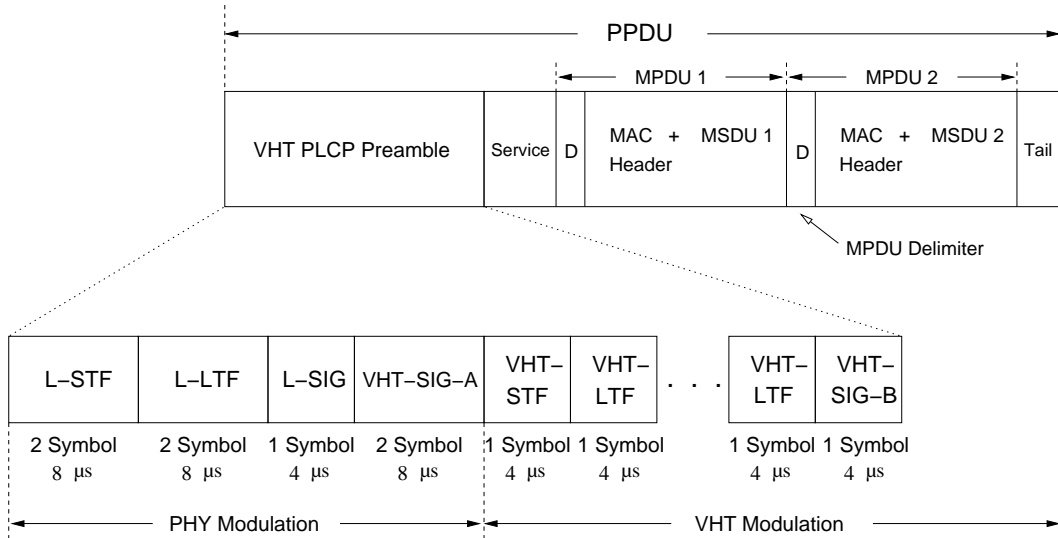
Fig. 1 PHY frame format of IEEE 802.11ac
