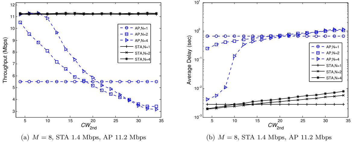
Fig. 10 Non-saturated throughput & Average delay
