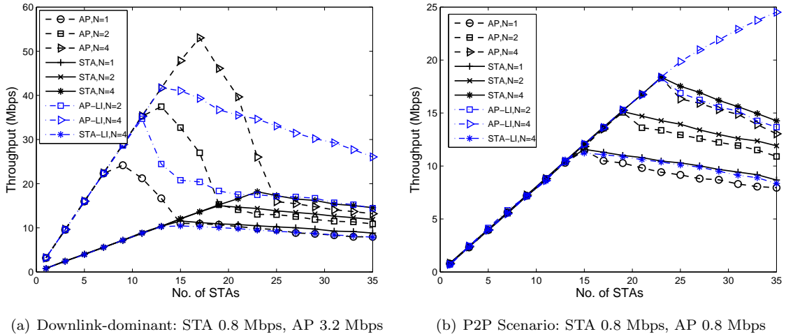
Fig. 13 Throughput against M
