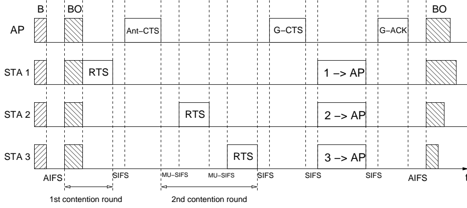
Fig. 5 A successful Uni-MUMAC uplink transmission
