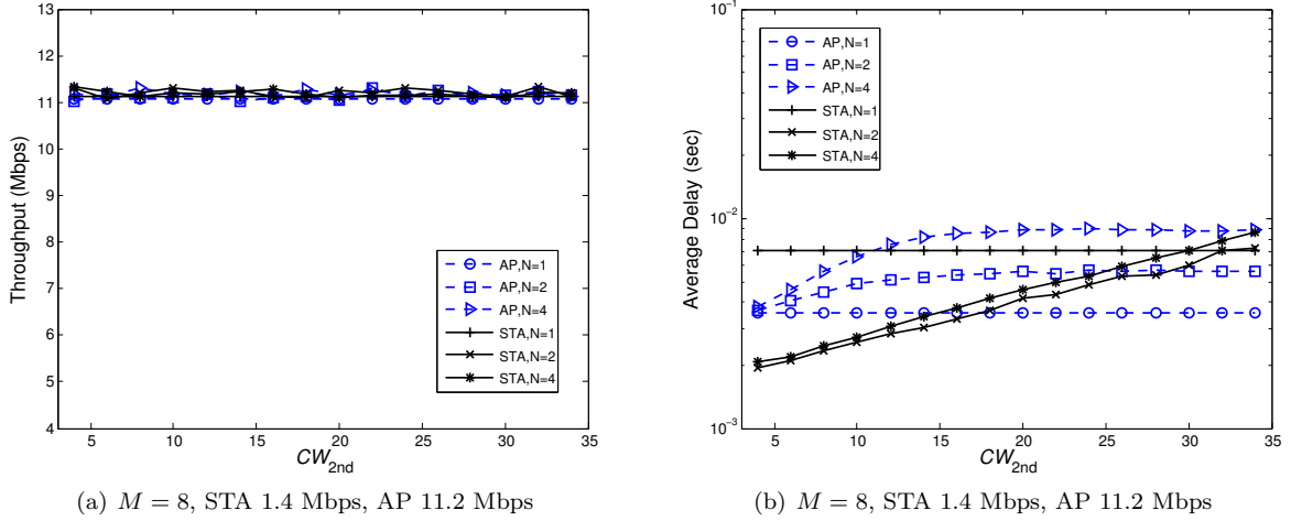
Fig. 12 Non-saturated throughput & Average delay when AP aggregates frames
