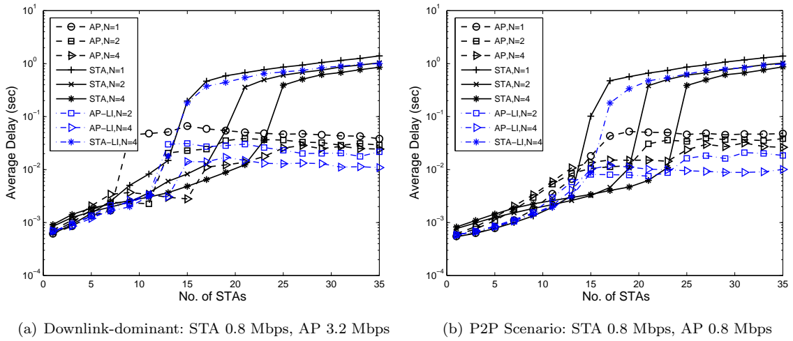
Fig. 14 Average delay against M
