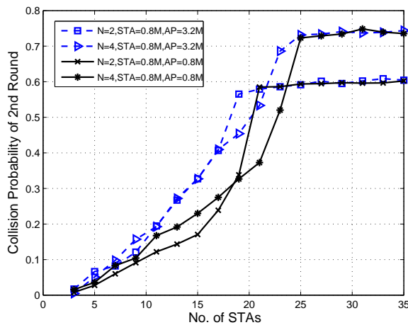
Fig. 16 2-nd round collision probability against M
