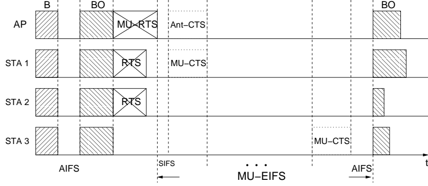
Fig. 6 Collisions in the 1-st contention round
