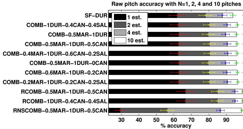
Figure 9: Mean raw pitch accuracy (RP) for the combination of four salience functions: DUR, MAR, SAL and CAN for N= 1, 2, 4 and 10 pitch estimates. Bars represent 95% confidence intervals. RCOMB denotes a combination with the proposed neighbour refinement method. RNSCOMB correspond to the refined estimation with the method proposed in (Duan, Pardo, and Zhang 2010). The values of \alpha are indicated before the name of each method. SF-DUR is shown as a reference.
