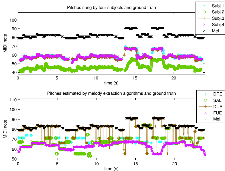
Figure 5: Pitches sung by four subjects and annotation of the melody, for an excerpt of the 4th movement of Dvořák’s 9th Symphony (top). Pitches estimated by four melody extraction methods and melody annotation for the same excerpt (bottom)
