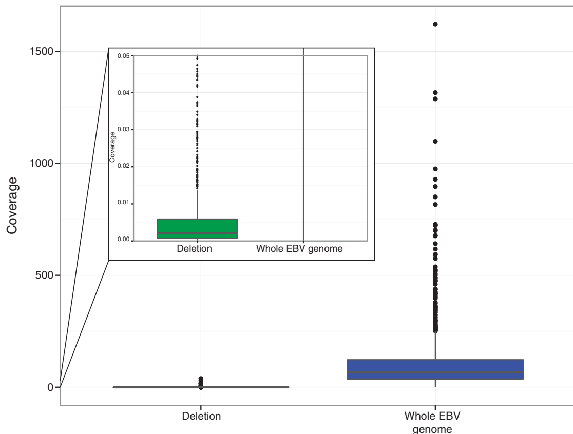
Fig. 1. —Boxplot of the coverage for all LCLs in the whole EBV genome (right) and in the B95-8-specific deletion (left). The inner panel displays a zoom in the coverage scale that shows that coverage at B95-8 is nonzero, suggesting the presence of natural EBV in some LCLs.
