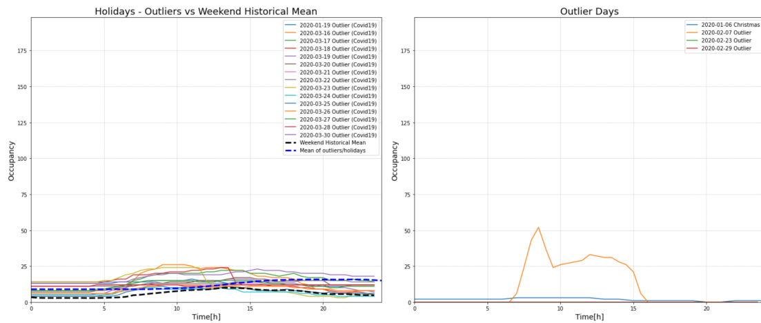
Figure 10: Comparison between the historical mean of Holidays and Outliers to the historical mean of Weekends on the left, and unjustifiable outliers in the right.
