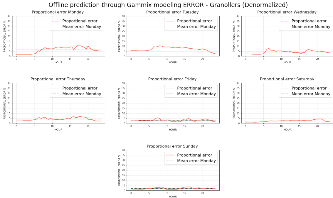
Figure 19: Proportional error of the prediction for each day of the week using Gammix prototypes in Granollers.
