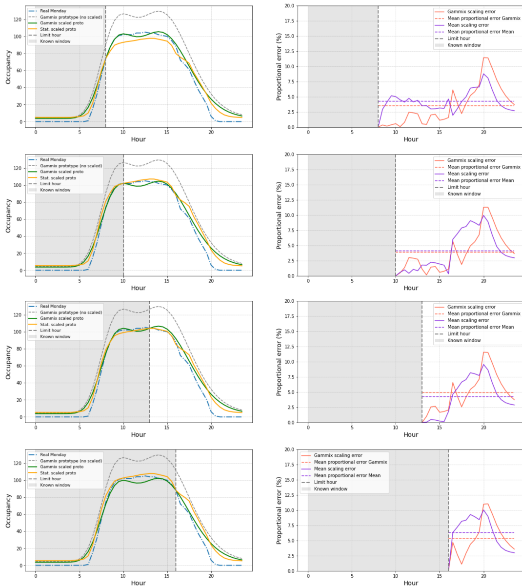
Figure 21: Prediction and proportional error of the remaining hours of a day given different times t=8,10,13,16 from top to bottom of an arbitrary testing Monday.
