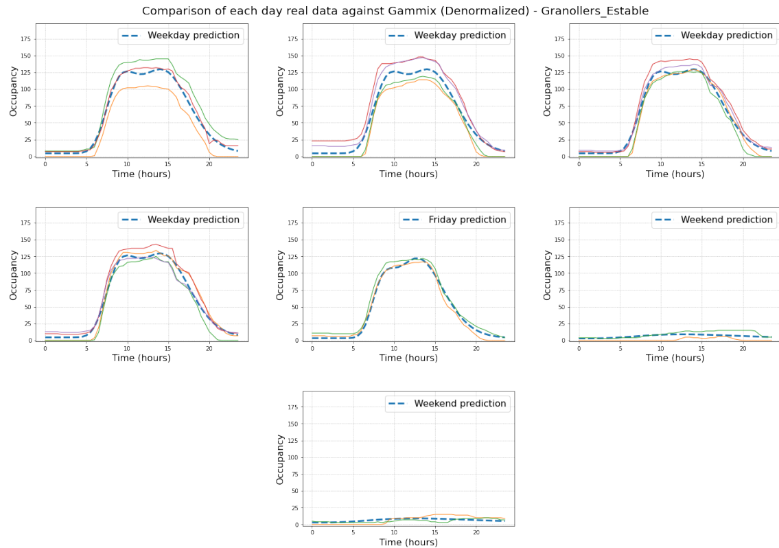
Figure 18: Comparison of the prediction using Gammix prototypes with testing days from Monday to Sunday.
