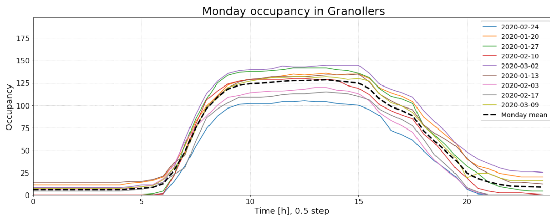
Figure 6: 24-hour occupancy cyclic behaviour for Mondays in the parking of Granollers.
