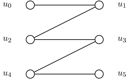
Figure 1: Illustration of the proof of Proposition 7 for k = 5 .
