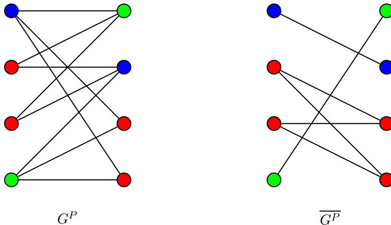
Figure 2: An example of G^P and \overline{G^P} from the proof of Theorem 8. The (vertex) colouring indicates the bicliques of \overline{G^P} .
