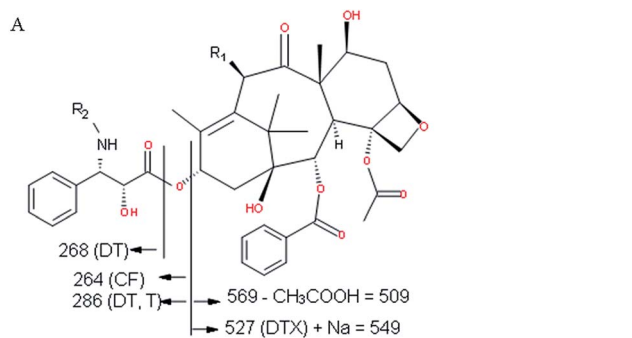
A) Common structure for taxol, 10-deacetyl taxol, cephalomannine and docetaxel T: R1 acetoxy group; R2 benzoyl group DT: R1: hydroxyl group; R2: benzoyl group CF: R1: acetoxy group; R2: N-Tigloyl group DTX: R1: hydroxyl group; R2: tert-Butyloxycarbonyl
