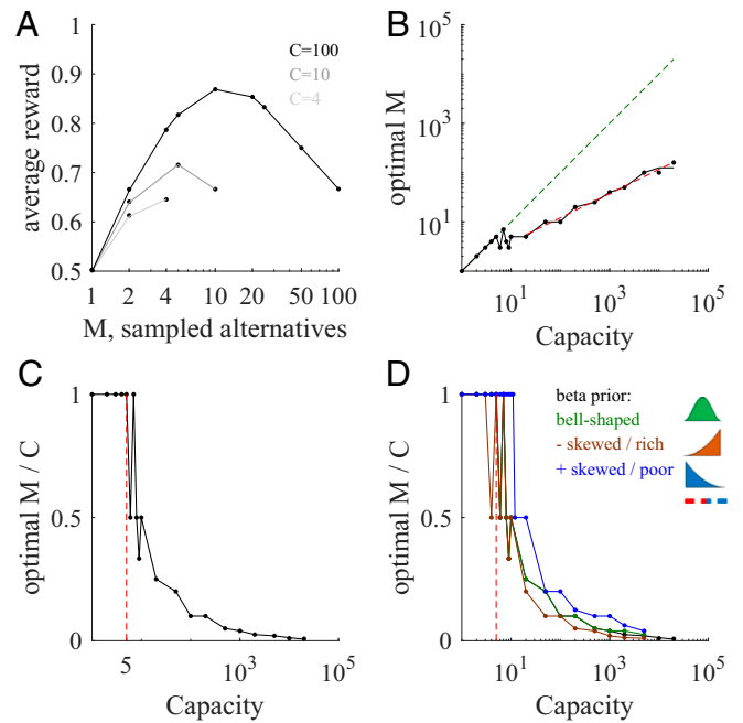
Fig. 2. Sharp transitions in optimal number of sampled alternatives at low capacity, and power law behavior at large capacity. (A) Average reward (points, simulations; lines, theoretical expressions; Eq. 4) as a function of the number of sampled alternatives M for three different capacities ( C = 4, 10, 100 ; light, intermediate, and dark lines, respectively) for the flat environment (uniform prior). The maximum occurs at the large extreme for low capacity but at a relatively low value for large capacity. Note log horizontal scale. (B) Optimal number of sampled alternatives as a function of capacity. When capacity is smaller than around 5, a linear trend of unit slope is observed (dashed green line), but when capacity is above 7, a sublinear behavior is observed (dashed red line corresponds to the best power law fit, with exponent close to 1/2). The black line corresponds to analytical predictions. The jagged nature of this prediction and simulation lines in this and other panels is due to the discrete values that the optimal M can only take, not due to numerical undersampling. (C) The sharp transition is clearer when plotting the optimal number of sampled alternatives to capacity ratio as a function of capacity. For low capacity, the ratio is 1, but for large capacity the ratio decreases very rapidly. The last point below which the optimal ratio is always 1 (critical capacity) corresponds to capacity equal to 5 (indicated with a vertical red line). (D) Number of sampled alternatives to capacity ratios for different prior distributions ( \alpha = \beta = 3 , bell-shaped, green line; \alpha = 3, \beta = 1 , negatively skewed prior modeling a “rich” environment, brown line; \alpha = 1, \beta = 3 , positively skewed distribution modeling looking for a “needle in a haystack,” that is, a “poor” environment, blue line). Lines correspond to analytical predictions from SI Appendix , Eq. 9; points correspond to numerical simulations; error bars are smaller than data points in all panels.
