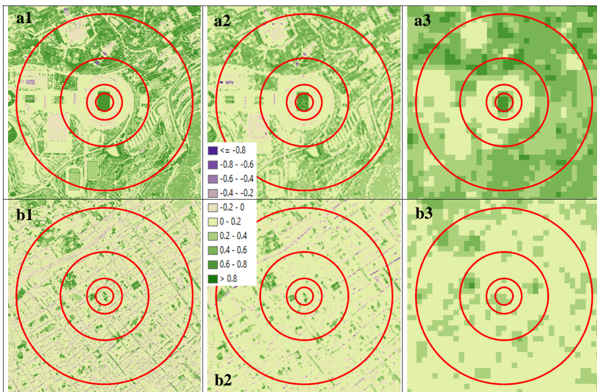
Fig. 3. NDVI surfaces and mean values in buffer sizes of 50, 100, 250 and 500 m (red circles) derived from WorldView2 (a1 for 0.59, 0.21, 0.20 and 0.25; and b1 for 0.10, 0.08, 0.07 and 0.07), RapidEye (a2 for 0.48, 0.17, 0.17 and 0.21; and b2 for 0.12, 0.09, 0.09 and 0.08) and Landsat8 (a3 for 0.60, 0.28, 0.29 and 0.34; and b3 for 0.18, 0.17, 0.18 and 0.17) for points of Estadi Olímpic (a) and Jardins del Mestre Balcells (b) vegetation cover areas in the immediate neighborhoods. (For interpretation of the references to colour in this figure legend, the reader is referred to the web version of this article.)
