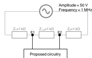
Figure 5. Setup used to demonstrate and evaluate the generated low frequency currents.
