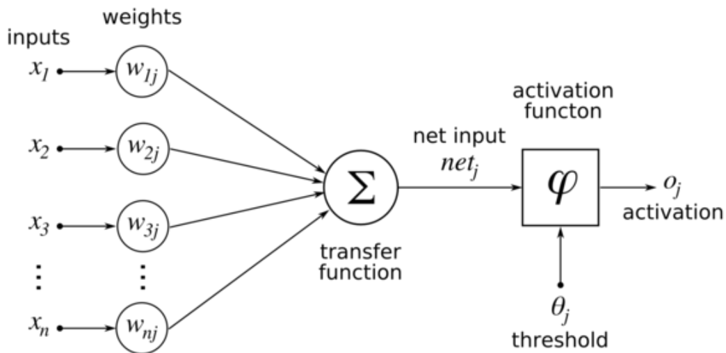
Figure 9: Components of an artificial neurone
