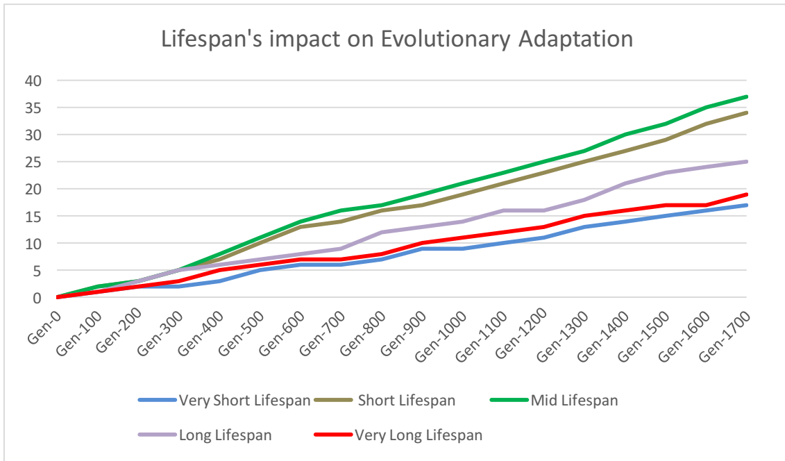
Chart 9: Lifespan's impact on Evolutionary Adaptation
