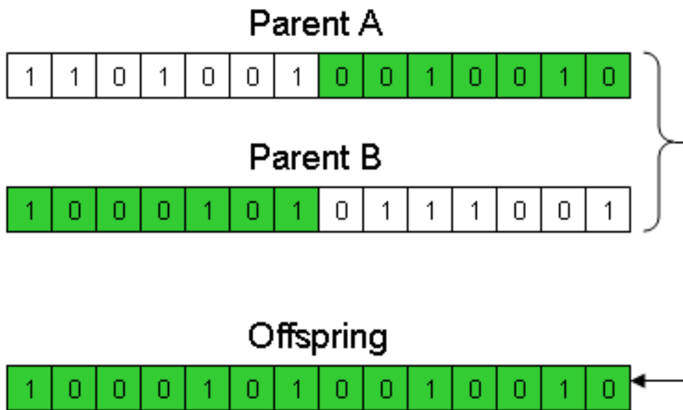
Figure 7: Artificial Representation of Genetic Crossover
