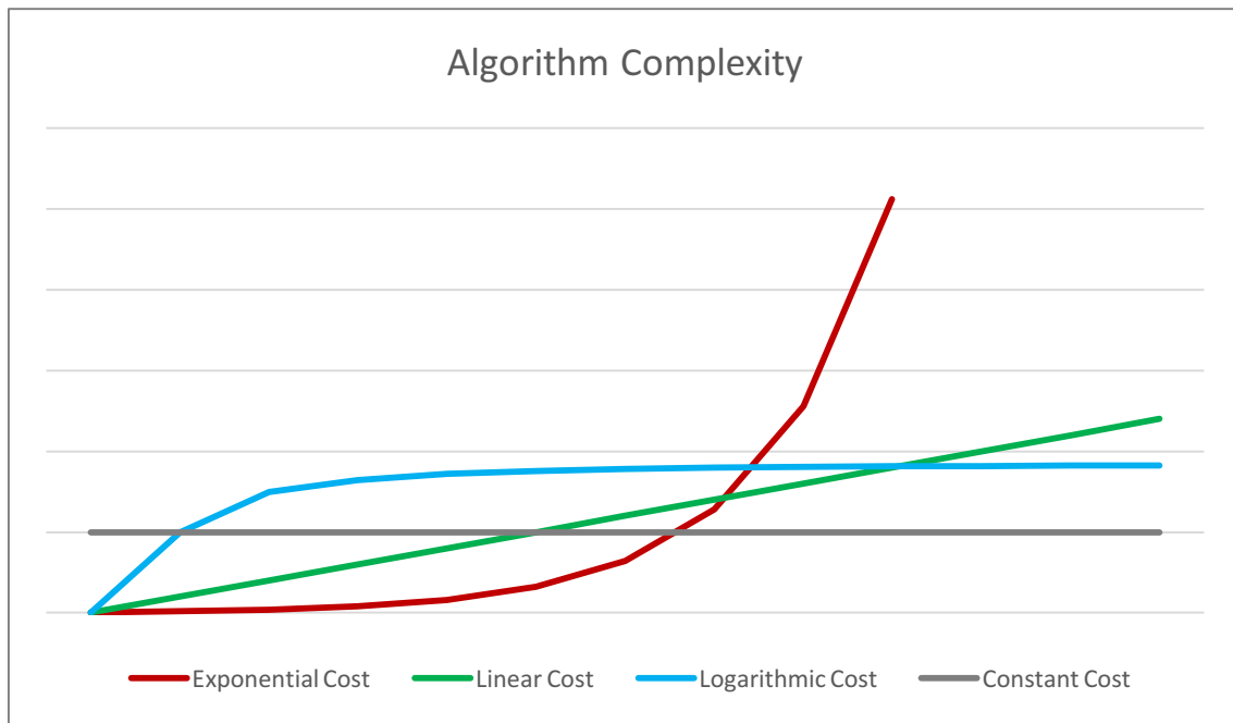
Chart 2: Algorithm Complexity
