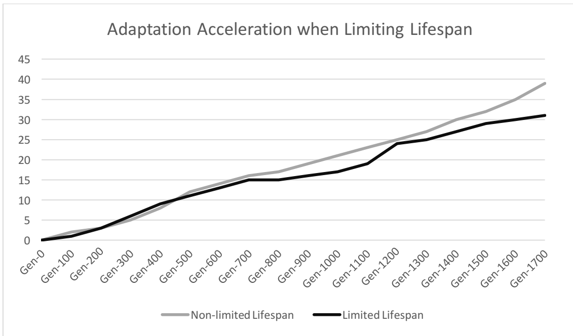
Chart 8: Adaptation Acceleration when Limiting Lifespan
