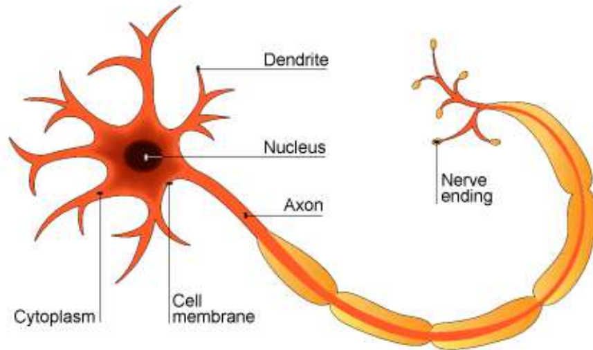
Figure 8: Components of a biological neurone
