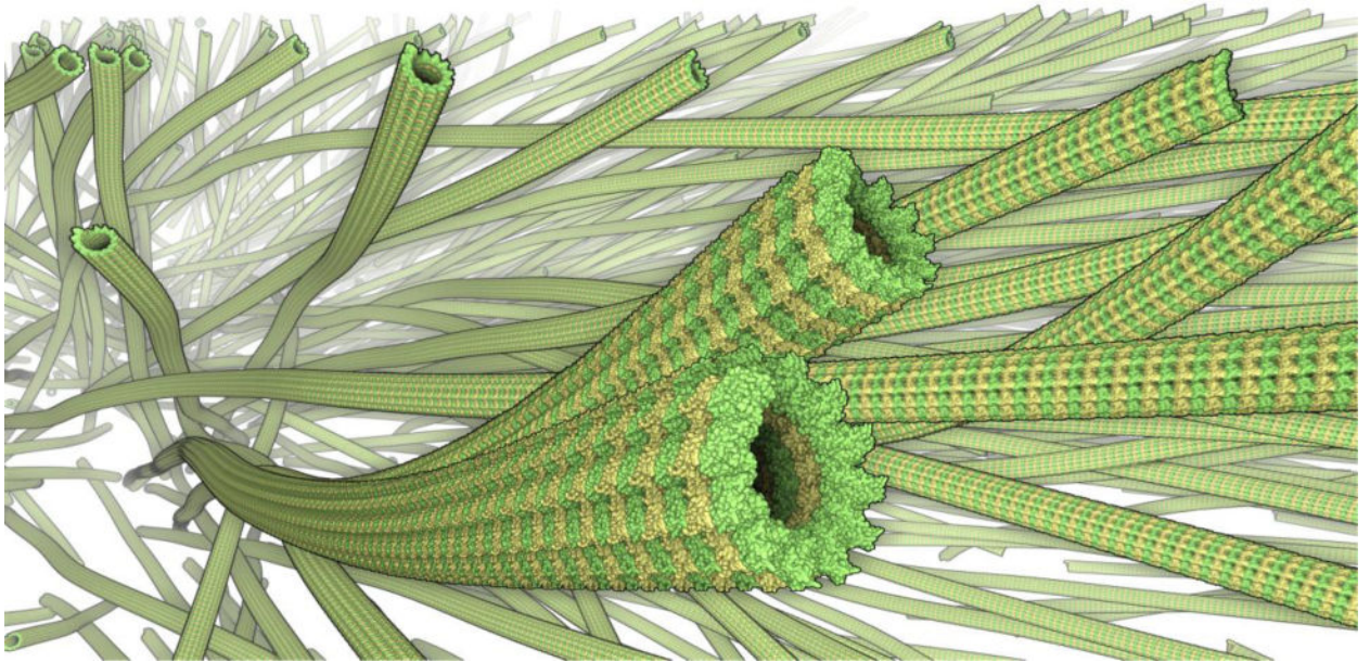
Fig 18. Visualization of microtubules (reconstructed from electron tomography data) containing about 10 billion atoms; rendered on commodity PC with subsecond framerate. The image is based on ref. (Lindow et al., 2012b).
