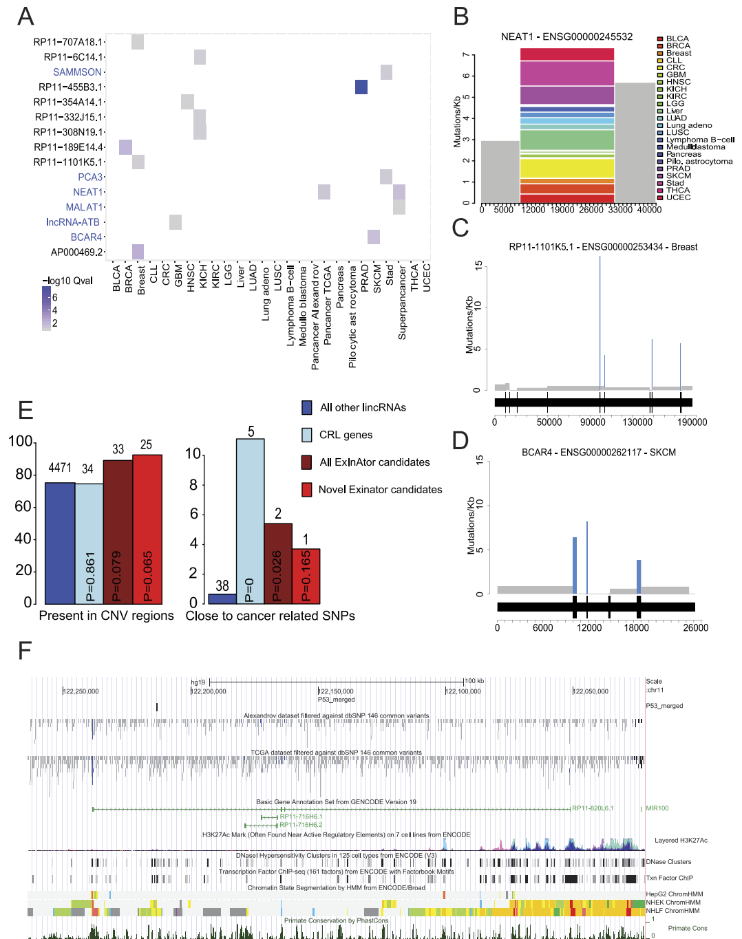
Figure 3. LncRNA cancer driver genes predicted by ExInAator across cancer genomes. (A) All driver lncRNAs ( Q \leq 0.1 ) and the tumour type in which they are identified. Gene names in blue indicate those belonging to CRL. (B) A mutation density plot for NEAT1 in all cancers, plotting the SNVs per kilobase as a function of gene regions. Grey represent background regions, while colours represent the mutational contribution of each cancer type to the single exon. The x-axis represents position, in bp, with respect to the start of the background region, defined here to be at 10 kb upstream of the gene's annotated TSS. (C) The Breast mutation profile of RP11-1101K5.1, a gene with mutations in four exons. Rectangles depict mutational density of exons (blue) and introns (grey). The gene structure is indicated below, where wider portions represent exons, separated by narrower introns. (D) The Breast mutation frequency in BCAR4. (E) Percentage of genes and candidates in CNV regions and proximal to cancer-related germline SNPs. Numbers above bars indicate the absolute numbers of genes represented by each percentage. Statistical significance in each case was estimated using Fisher's Exact test. (F) An example of an ExInAator-predicted novel candidate gene, RP11-820L6.1. Note the presence of promoter-like histone marks (red, ChromHMM track), evolutionary conservation (PhastCons Primate conservation), and cancer SNVs around the gene TSS, as well as a proximal P53 binding site ("P53_merged").
