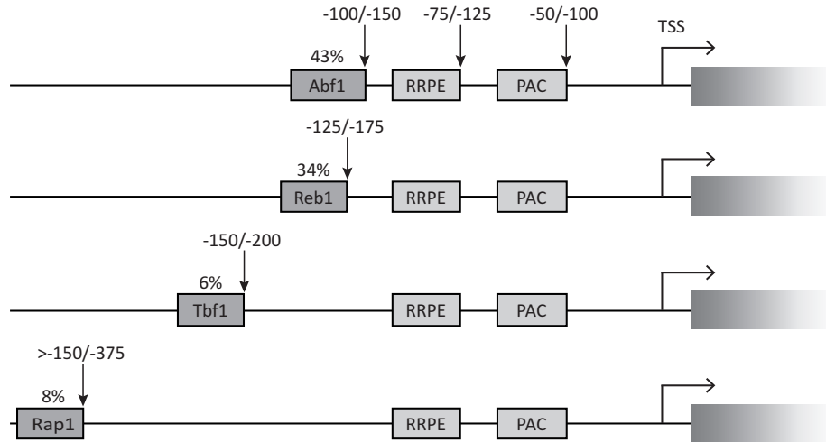
Figure 1. Conserved sequence elements in Saccharomyces Ribi gene promoters. Graphical representations of promoter architecture of Ribi genes as derived from in silico analysis. The ~20% of Ribi genes which did not display any conserved GRF binding site is not represented in the Figure. Indicated above each GRF box is the percentage of Ribi gene promoters in which the motif occurs. Vertical arrows pointing to the downstream end of the boxes are to indicate their range of distances (in base pairs) above the arrows) with respect to the TSS. The consensus sequences considered for the different elements reported are: PAC, GCGATGAGMT; RRPE, TGAAAAWTTTY; Abf1, RTCAYNNNN(N)ACGR; Reb1, RTTACCCK; Tbf1, ARCCCTAA; Rap1, WACAYCCRTACATY (M, A or C; W, A or T; R, A or G; Y, C or T; K, G or T; N, any nucleotide). These consensus sequences are based on the following references: PAC and RRPE (1); Abf1 (10,12,55); Reb1 (10,55); Tbf1 (10,12,18); Rap1 (56).
