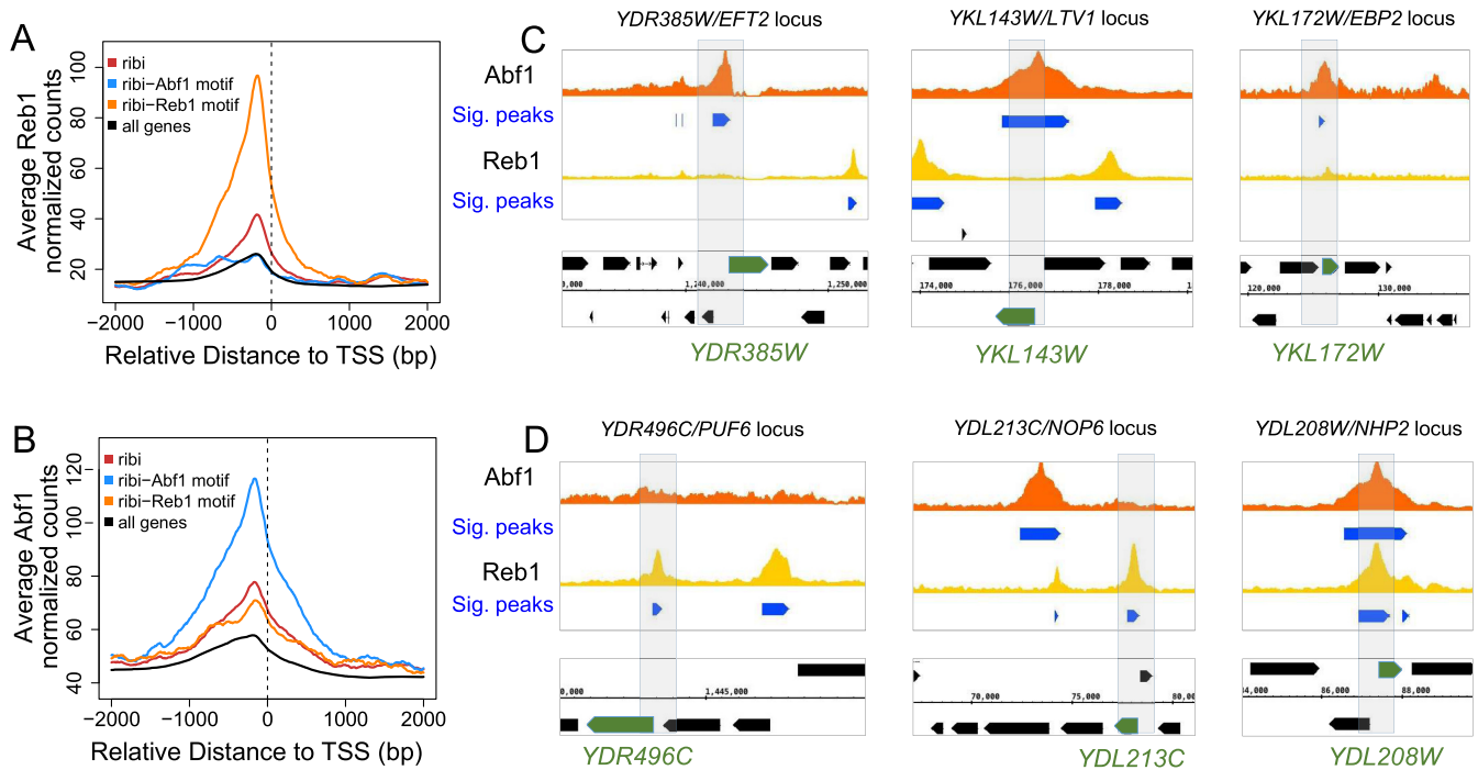
Figure 2. In vivo association of Abf1 and Reb1 to Ribi gene promoters. (A) Average binding profiles (normalized total counts) of Reb1 across the TSS regions of annotated yeast promoter regions for different set of gene lists as indicated in the inset (see text and Supplementary material). (B) Average binding profiles (normalized total counts) of Abf1 across the TSS regions of annotated yeast promoter regions for the same genes lists as in (A). (C) Genome browser plots showing normalized tags counts (and significant peaks in blue) of Abf1 and Reb1 binding for ribi genes ( EFT2 , LTV1 and EBP2 ) that showed significant enrichment for binding of Abf1 (but not Reb1). Bound gene is highlighted in green color. Relevant TF peaks and the corresponding Ribi genes are boxed. (D) Genome browser plots showing normalized tags counts (and significant peaks in blue) of Abf1 and Reb1 binding for Ribi genes ( PUF6 and NOP6 ) that showed significant enrichment for Reb1 binding (but not Abf1) and NHP2 , a Ribi gene whose promoter contains significant region of binding for both factors. Bound gene is highlighted in green color. Relevant TF peaks and the corresponding Ribi genes are boxed.
