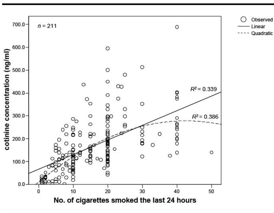
Figure 1 The distribution of salivary cotinine concentration in relation to the number of cigarettes smoked during the 24 hours prior to saliva collection.
