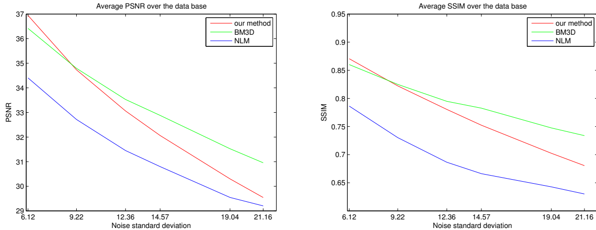
Figure 1. Average PSNR value (left) and SSIM index value (right) computed over our proposed image data base, for comparing our proposed local denoising method to BM3D and NLM denoising.
