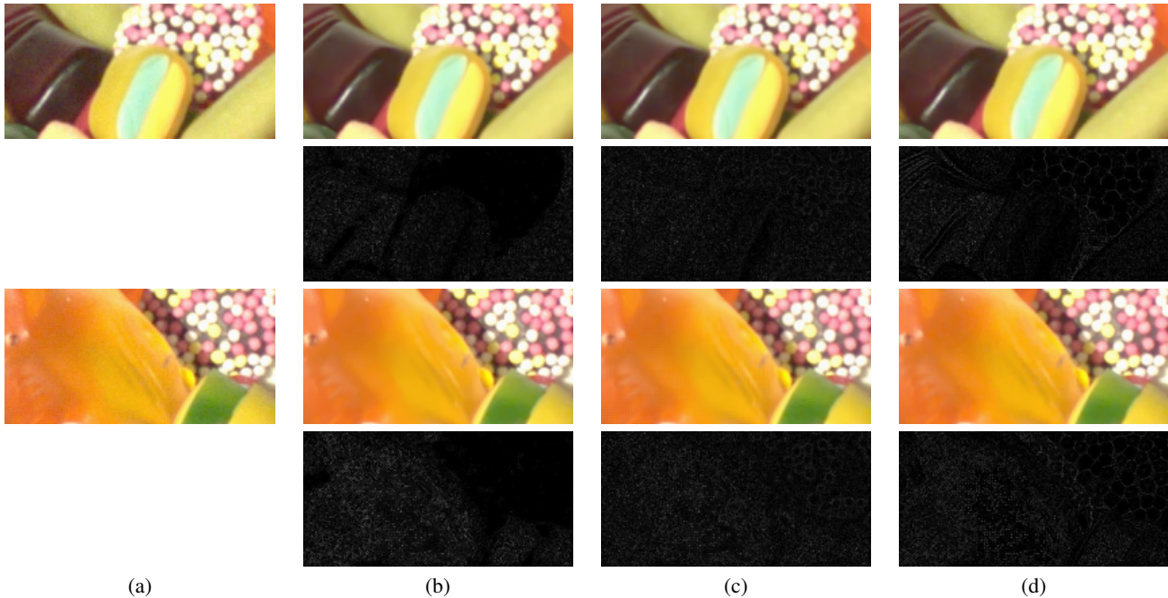
Figure 6. Comparison of our local denoising framework to NLM and BM3D denoising algorithms, for the ARRI pipeline. Row 1 and 3. (a) crop from noisy ARRI image "candy". (b) NLM result, PSNR=40.72. (c) BM3D result, PSNR=41.18. (d) our result, PSNR=40.20. Row 2. Noise difference images for crops of Row 1, scaled for visualization with a scaling factor 7 (b) NLM result. (c) BM3D result. (d) our result. Row 4. Noise difference images for crops of Row 3, scaled for visualization with a scaling factor 7 (b) NLM result. (c) BM3D result. (d) our result.
