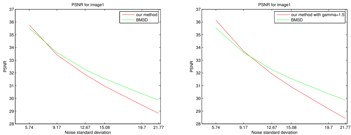
Figure 5. Left: PSNR value for “image1”, for comparing our proposed local denoising method to BM3D. Right: PSNR value for “image1”, for comparing our local denoising method with a gamma power of 1.5 to BM3D.
