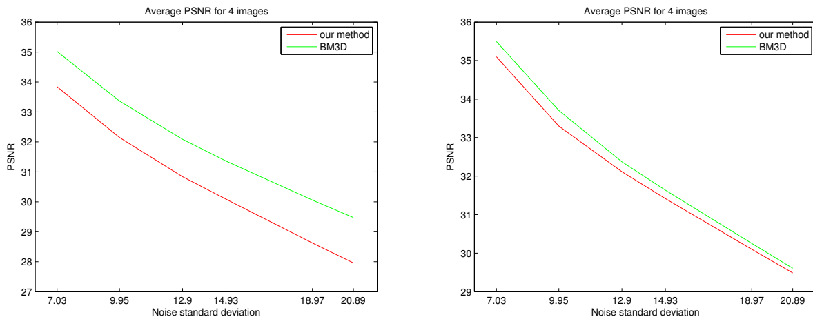
Figure 3. Left: Average PSNR value for 4 images from our data base, for comparing our proposed local denoising method on a 8-bit depth image to BM3D. Right: Average PSNR value for 4 images from our data base, for comparing our proposed local denoising method applied after the gamma-correction to BM3D.
