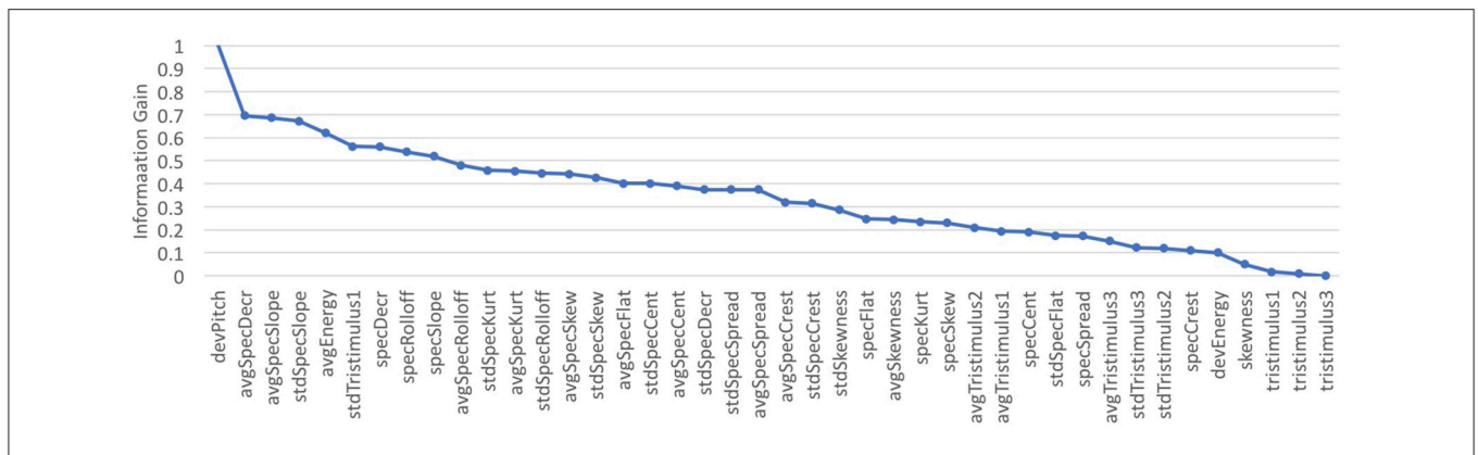
FIGURE 3 | Feature selection: Rankings based on information gain.
